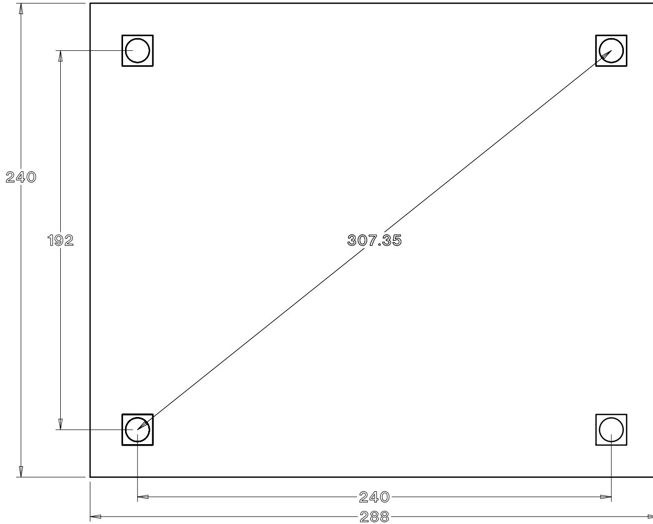
20 x 24 Fiberglass pergola
