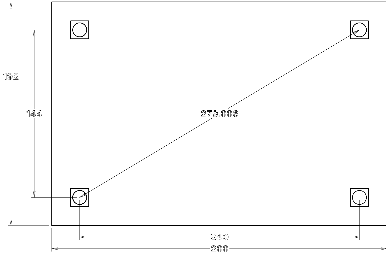
16 x 24 Fiberglass pergola
