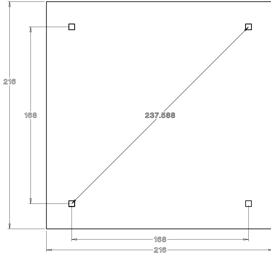
18 x 18 Post and beam pergola
