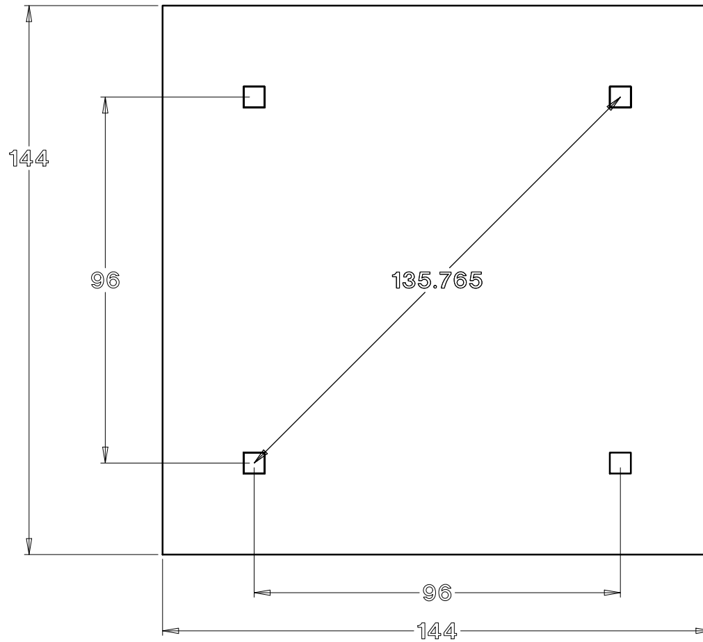
12 x 12 Post and beam pergola
